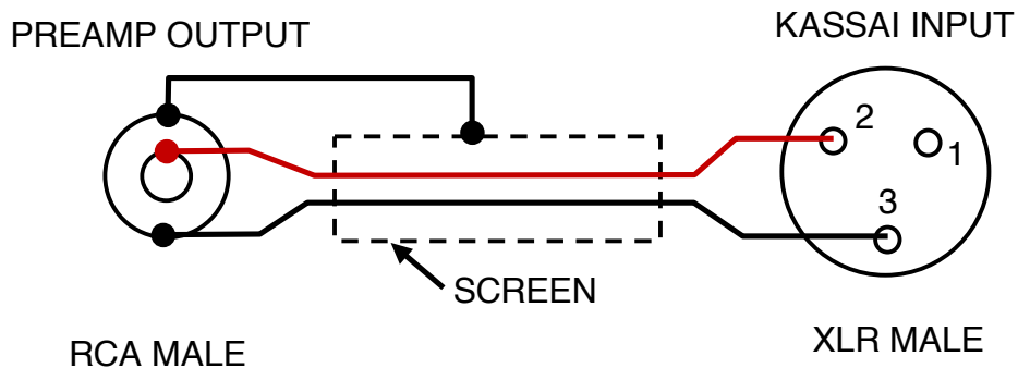
CABLE CONFIGURATION FOR RCA SINGLE ENDED PREAMP OUTPUT TO XLR BALANCED AMPLIFIER INPUT
