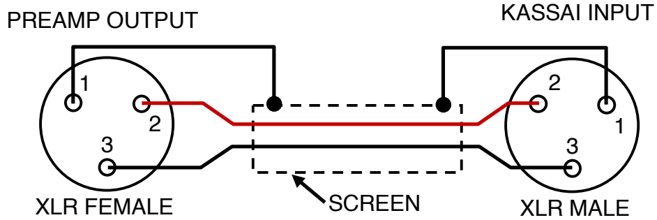
CONVENTIONAL: SCREEN CONNECTED AT BOTH ENDS
