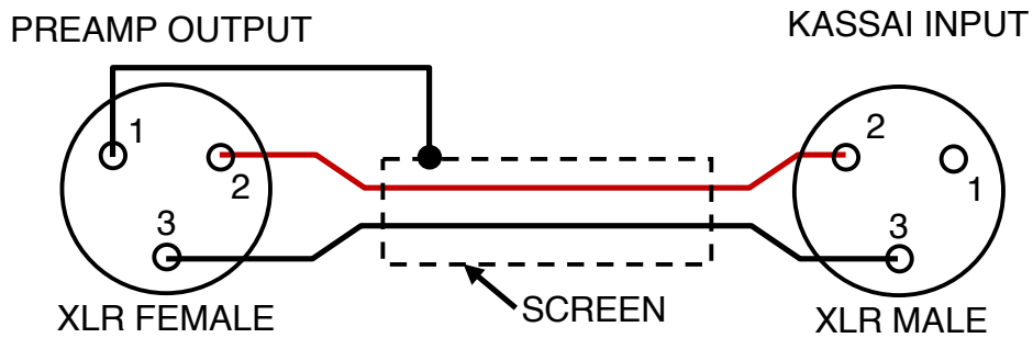
SCREEN CONNECTED AT PREAMP END ONLY, TO ELIMINATE GROUND LOOPS
