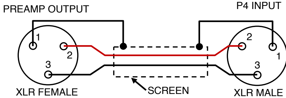
CONVENTIONAL: SCREEN CONNECTED AT BOTH ENDS
