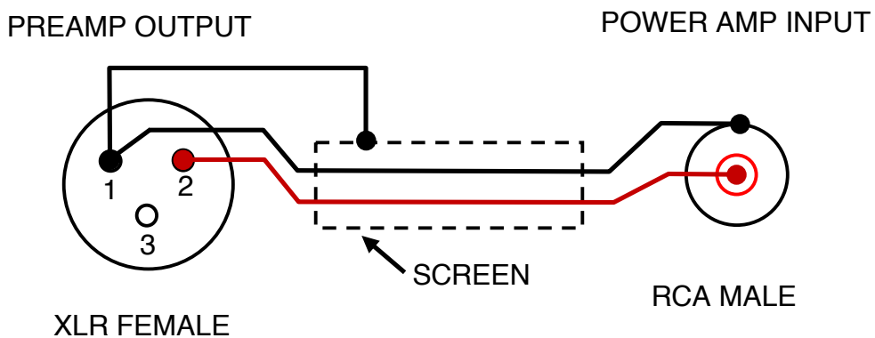
SCREEN CONNECTED AT PREAMP END ONLY, TO ELIMINATE GROUND LOOPS
