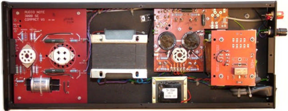
Photo 1: Internal top view of amplifier
