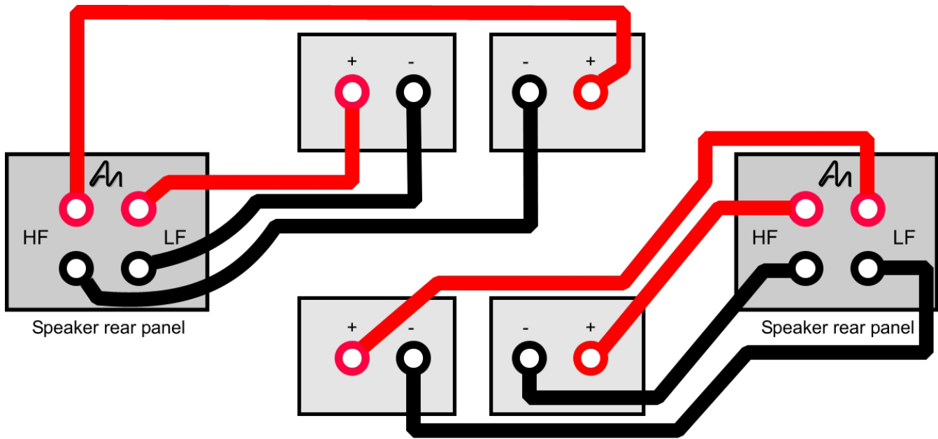
Figure 5 - Bi-amping with four mono amplifiers
