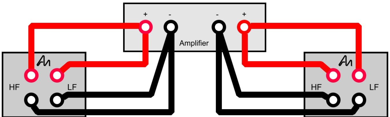
Figure 2 - Bi-wire connection with a single stereo amplifier
