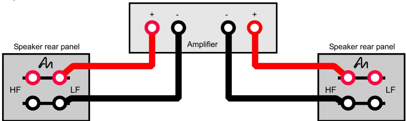
Figure 1 - Connection with a single stereo amplifier
