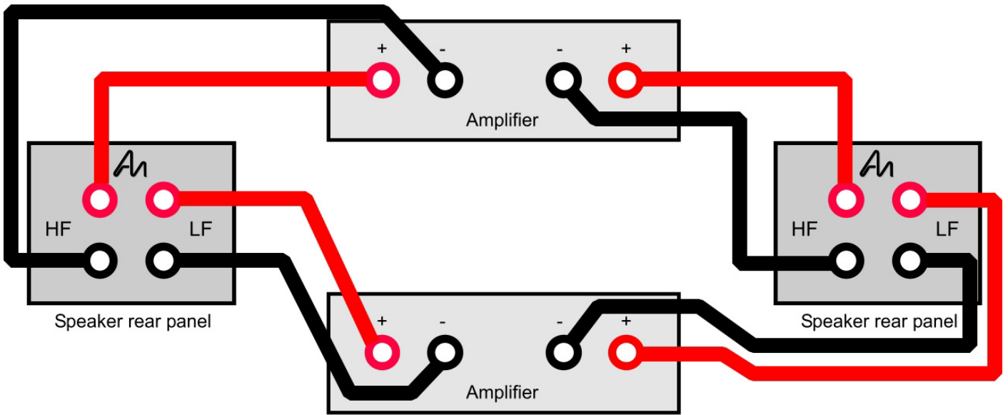
Figure 4 - Bi-amping with one stereo amplifier per drive unit for both channels
