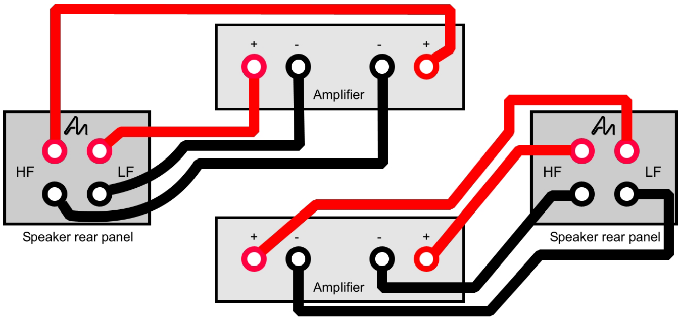
Figure 3 - Bi-amping with one stereo amplifier per channel
